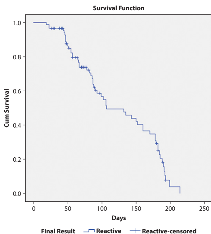
Means and Medians for Survival Time
