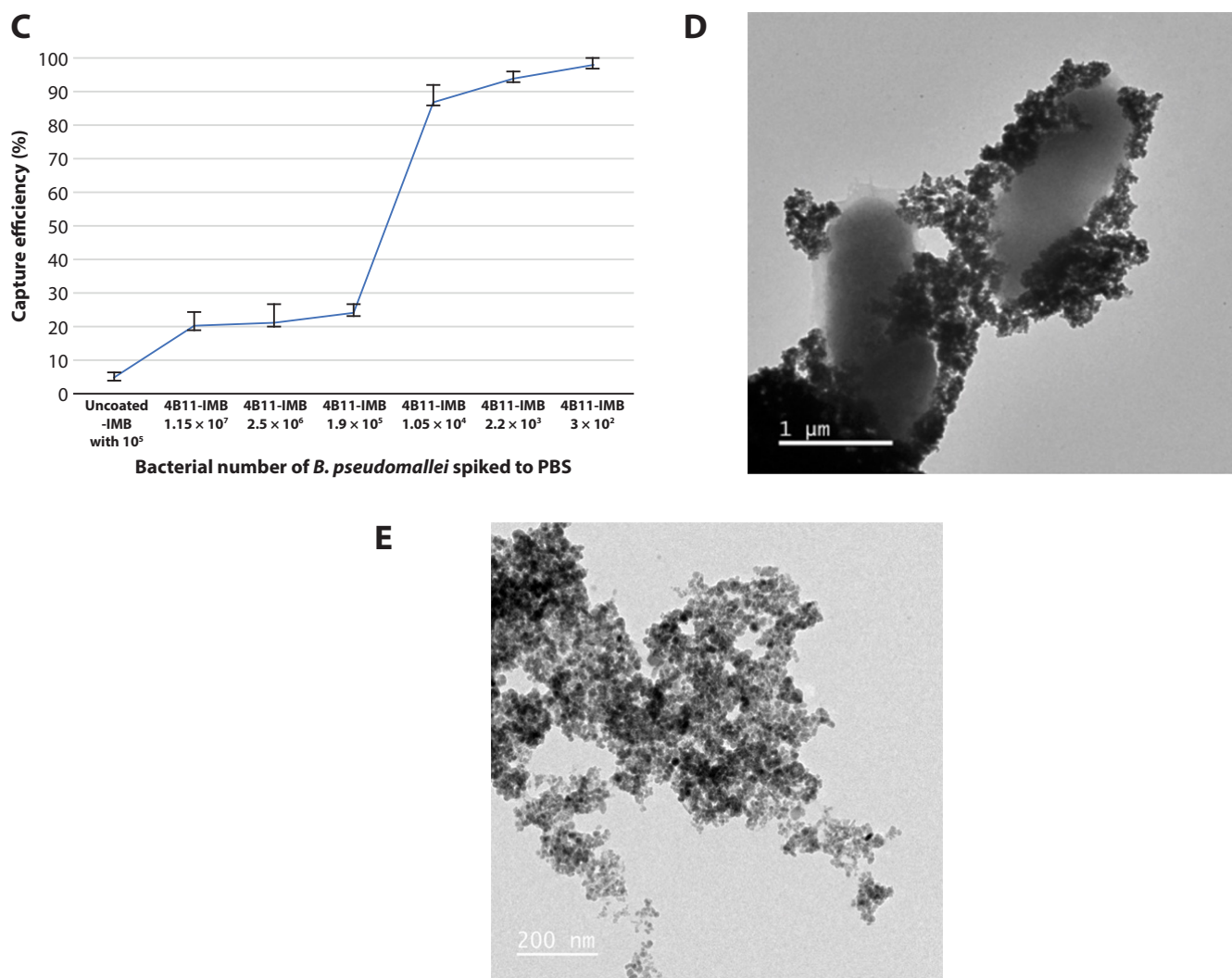
Figure 2. (Continued) The optimal coated-IMB (4B11-IMB) were evaluated for capture efficiency using 3 \times 10^2 , 2.2 \times 10^3 , 1.05 \times 10^4 , 1.9 \times 10^5 , 2.5 \times 10^6 , 1.15 \times 10^7 B. pseudomallei cells (C). The bound and unbound bacteria were measured by the culture method and the percentage of capture efficiency (CE) calculated to evaluate the ability of the bead for binding, capture and separation of bacteria. The line represents the mean of CE \pm SD. The uncoated-IMB used for capturing B. pseudomallei at 10^5 CFU/ml was used as a negative control. TEM image of the F200 IMB-bound B. pseudomallei in buffer (PBS) (D). The negative control beads are shown (E).
