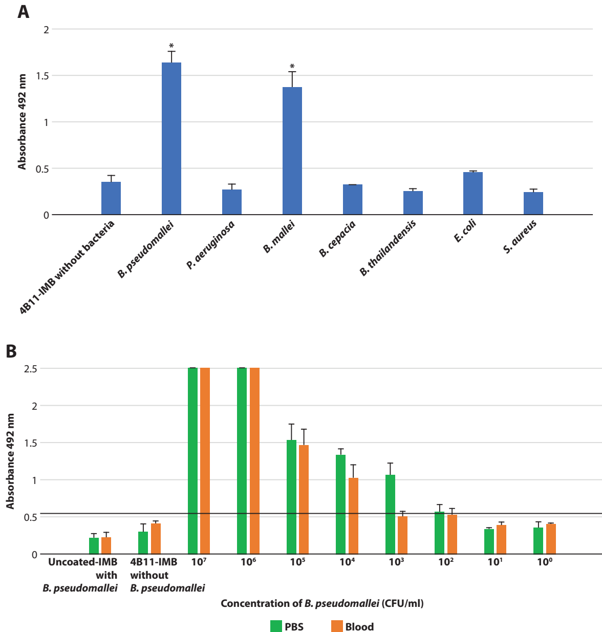
Figure 3. Specificity and sensitivity of IMB-ELISA for detection of B. pseudomallei . For the specificity test, 10 5 CFU/ml of various bacteria were spiked into 1ml EDTA blood and detected by IMB-ELISA while the 4B11-IMB without bacteria was used as the negative control (A). Each bar represents mean ± SD. The asterisks (*) indicate statistical significance (p < 0.05) compare to control. Sensitivity of IMB-ELISA was tested for detection of B. pseudomallei in buffer compared with inoculated blood samples (B). The B. pseudomallei was 10-fold serially diluted from 10 0 to 10 7 CFU/ml into 1 ml of PBS buffer and EDTA blood prior for detection by using IMB-ELISA. The negative control groups included uncoated-IMB with 10 5 CFU/ml of B. pseudomallei and 4B11-IMB without bacteria. The absorbance by the ELISA reader was at 492 nm. Each bar represents mean ± SD. The line represents the cut off (Mean of 4B11-IMB without bacteria plus 3 SD) of the IMB-ELISA test.
