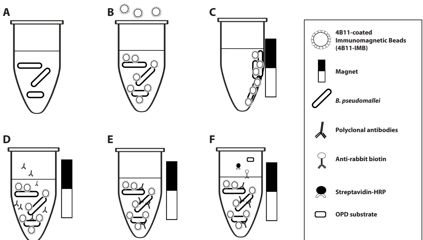
Figure 1. Schematic illustration of the system for detection of Burkholderia pseudomallei by IMB-ELISA. Bacteria in 1 ml of blood samples in microtubes (A) were captured by 4B11-IMB (B). After incubation for 1 h, the bacteria-bound beads were separated by magnetic force (C) and the unbound substances were removed from the reaction. The secondary (PAB) against B. pseudomallei were then added and incubated for 30 min (D) followed by removing the excess antibodies (E). The conjugated antibodies (biotinylated anti-rabbit antibodies and streptavidin-HRP) were added (F) for detection by ELISA.
