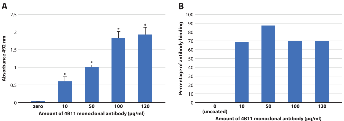
Figure 2. The optimization of coating antibodies for MAb-coated IMB. The various concentrations of 0, 10, 50, 100 and 120 \mu g/ml of monoclonal antibody 4B11 were coated on beads and concentrations of bound antibodies were determined by ELISA (A). Each bar represents mean \pm SD of the absorbance of antibody coated on the beads. The asterisks (*) indicate statistical significance ( p < 0.05 ) compare to control. The percentage of antibody binding was calculated by the percent of the amount of antibody added minus the amount of antibody left divided by the amount of antibody added (B).
