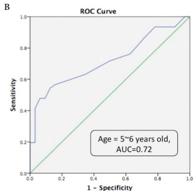
Figure 2. Receiver operating characteristic (ROC) curves were constructed in different age groups. (A) Children aged 5 to 18 years (FeNO \geq 20.5 ppb, area under the ROC curve[AUC][95%CI]0.78[0.74-0.82]); (B) Children aged 5 to 6 years (FeNO \geq 15.5 ppb, AUC 0.72[0.61-0.83]);
