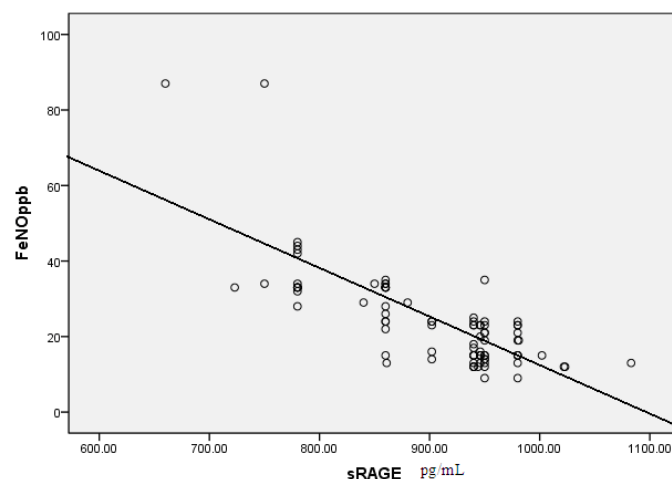
Figure 3. Spearman's rank correlation test showed that there was correlation between FeNO and sRAGE in children with recurrent wheezing.
